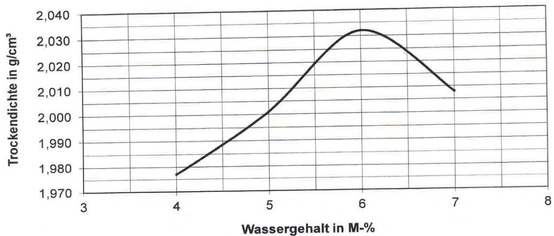
Proctorkurve 0/32 mm
